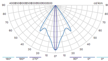
6286 - Diffuser P25 striated
