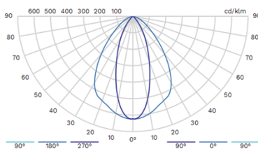
6290 - Diffuser P25 striated
