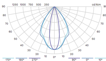
6289 - Diffuser P25 striated
