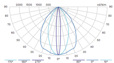
6291 - Diffuser P25 striated
